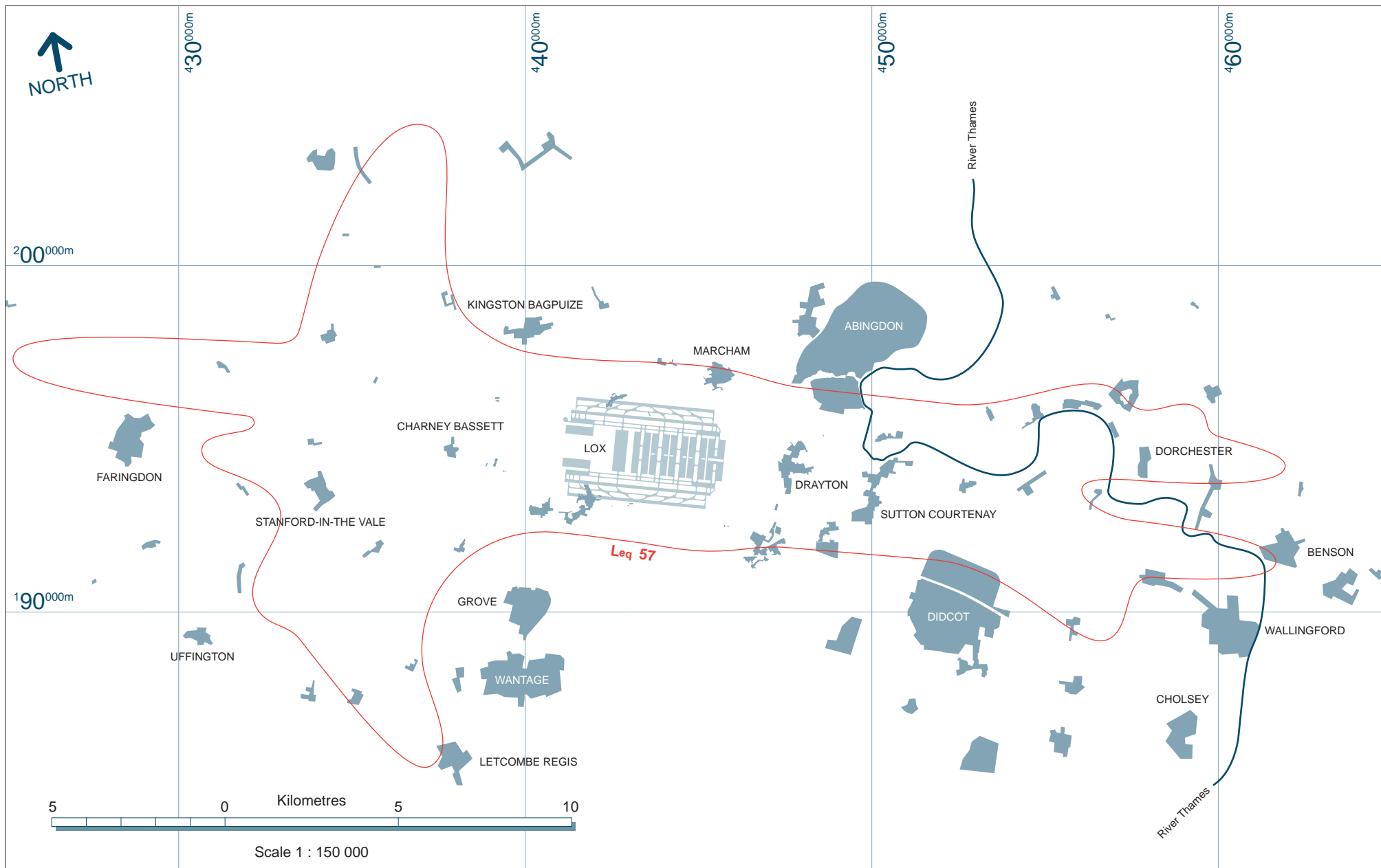
Figure 10 Leq 57 dBA noise contour (2040)
